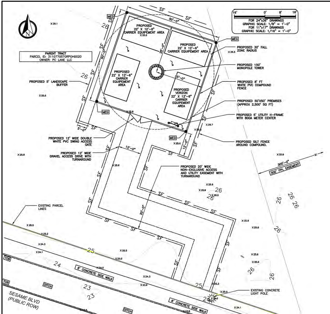
Figure 6. Ground Compound Plan
