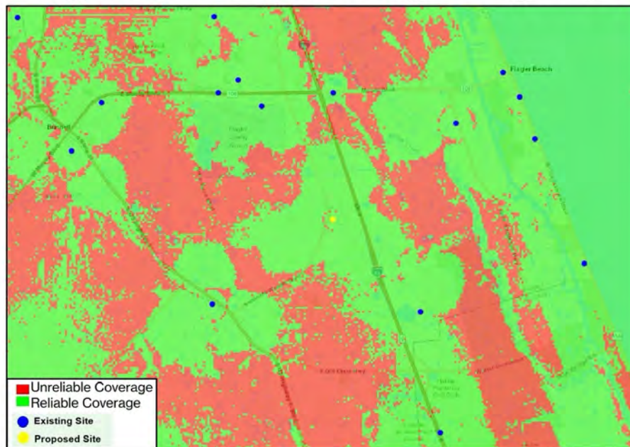
Figure 3. Verizon Propagation Maps
