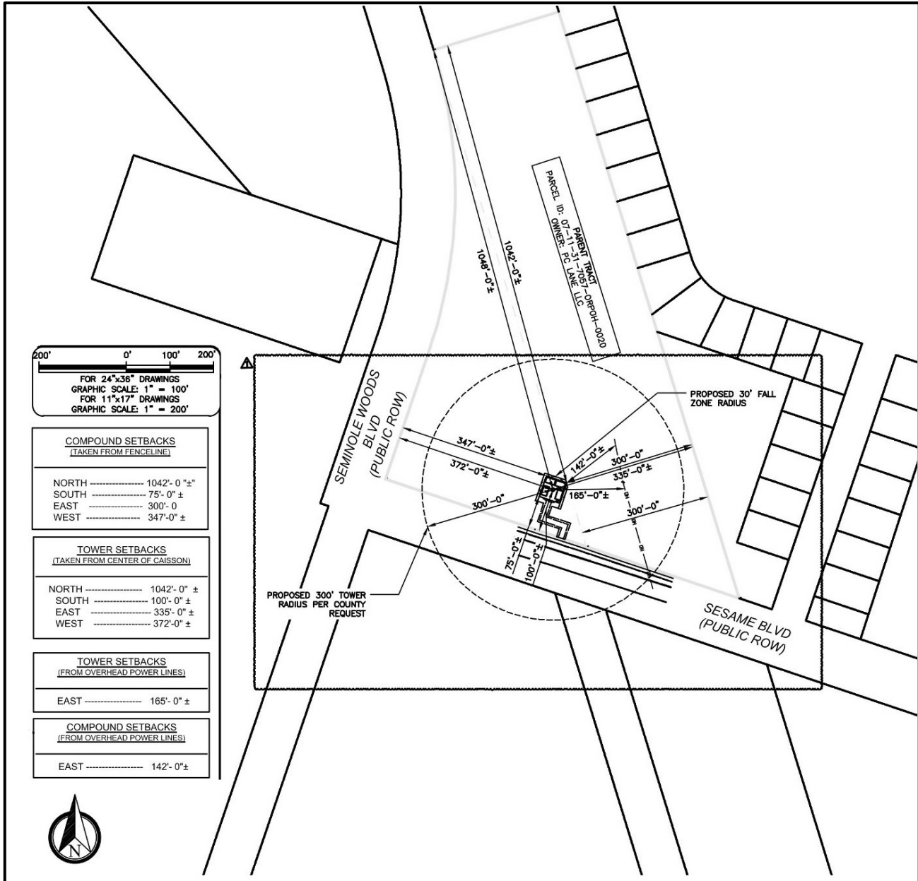
Figure 5. Tower & Compound Setbacks
